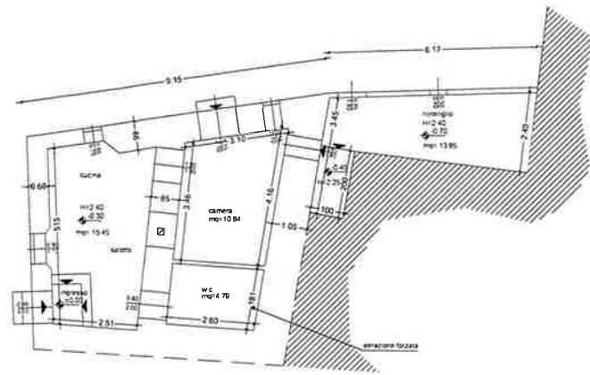
PIANO TERRA (approvato CTE 11326) scala 1:50
